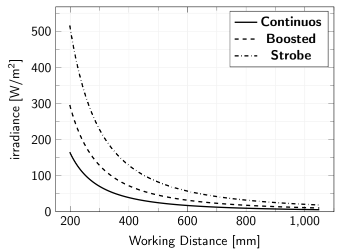
Irradiance Characteristics
